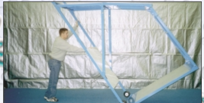
Tip unit up into place and attach launchers and bumpers.
