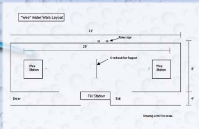
Space Requirements
